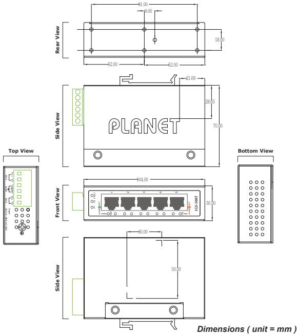
Figure 1: IGS-500T Three-View Diagram
