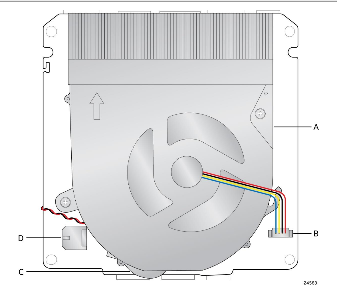
Figure 2. Major Board Components (Top)
