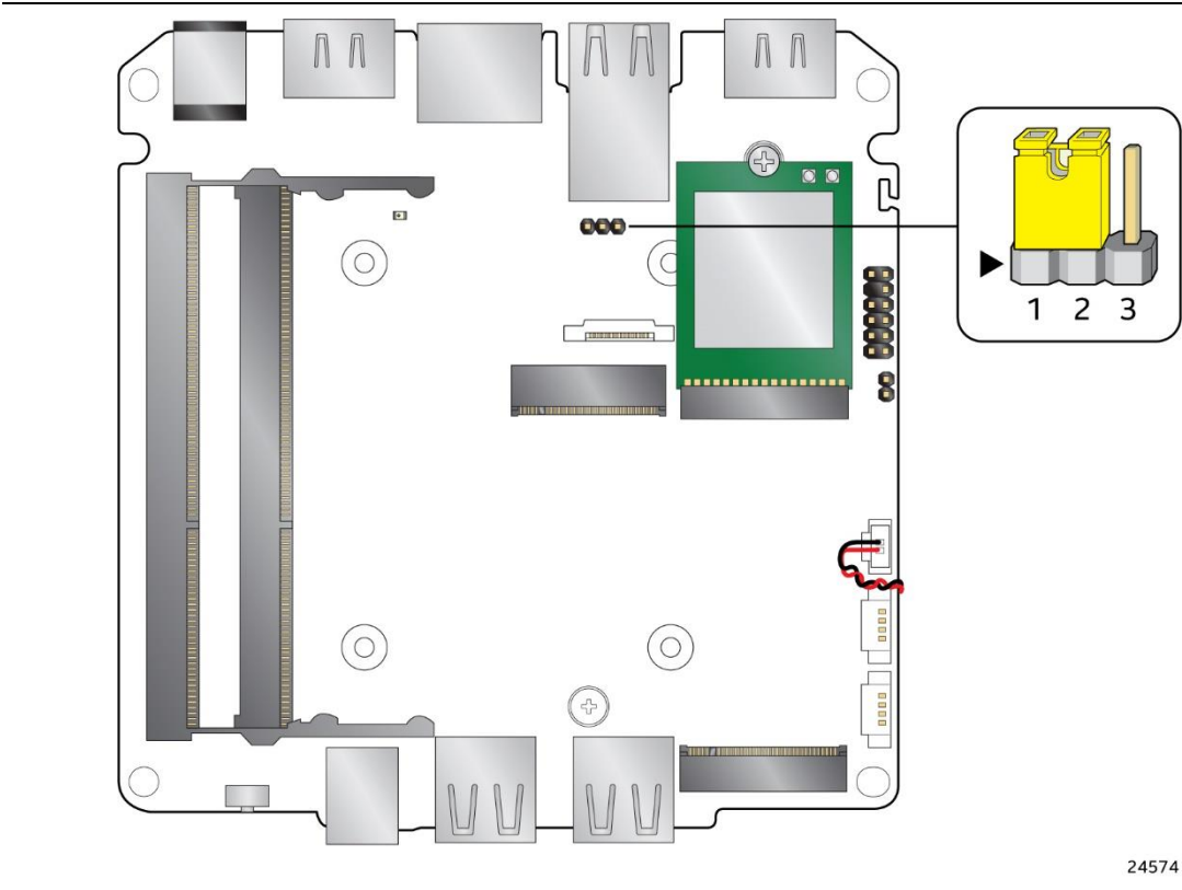
Figure 9. Location of the BIOS Security Jumper
